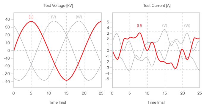
Fig. 4 Test voltage and current waveform – no-load loss measurement at 100 % with THDu < 3.2 % and THDi = 43 % (500 MVA transformer)
