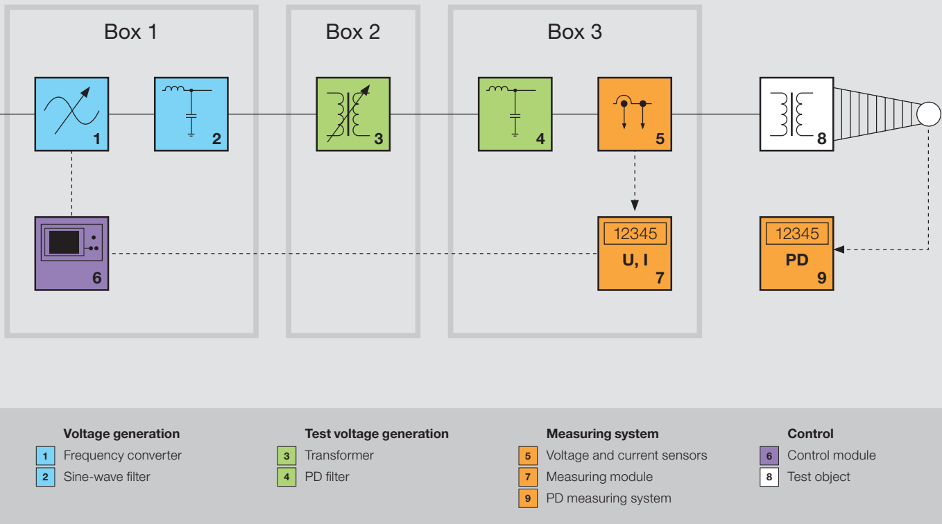
Fig. 2 Block diagram of test source WV 18-18/1.4
